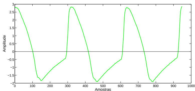
Figura 5.2: Sinal EGG
